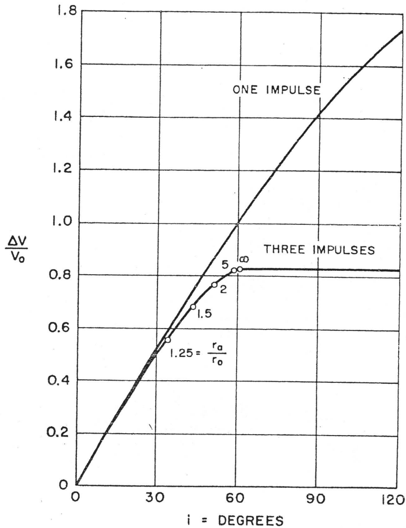
Fig. 6.12 Transfers between Inclined Circular Orbits of Equal Radius (Copyright, 1966, American Institute of Aeronautics and Astronautics; reprinted with permission)
