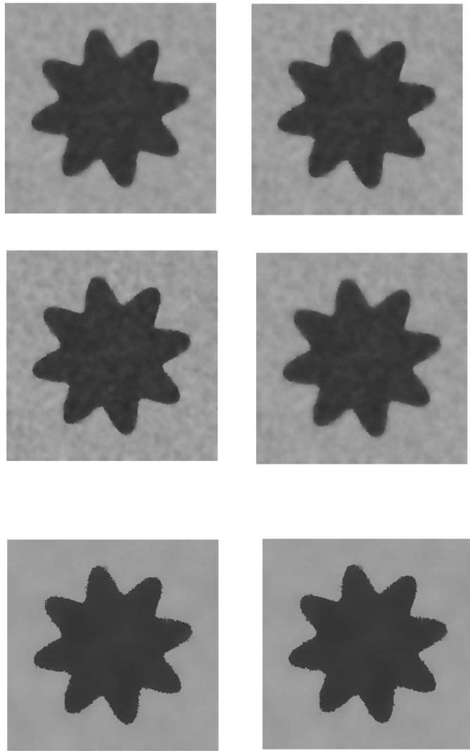
Figure 3. Pictures shows the work for parameter K = 100 (top) for different scale steps k = 1, 2, 5, 10 , and for parameter K = 1000 for scale parameter k = 10, 20 for Example 2.
