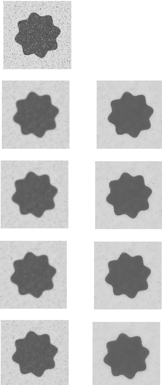
Figure 1. The first column shows the work for parameter K = 10 for different scale steps k = 0.1, 0.5, 1, 2.5. , the second column shows the work for parameter K = 100 for scale steps k = 0.5, 1, 4, 10. for Example 1.
