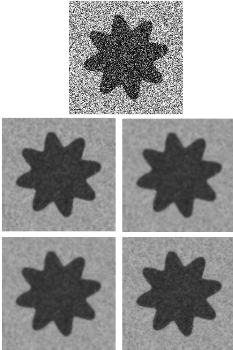
Figure 2. Pictures shows the work for parameter K = 10 for different scale steps k = 0.2, 1, 5, 10 (from the top to bottom, from left to right) for Example 2.
