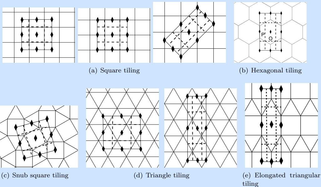
Figure 10. FVT actions of the group pgg .
