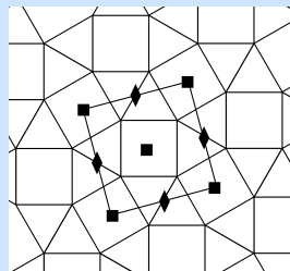
(b) Snub square tiling
