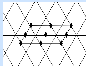
(b) Triangle tiling
