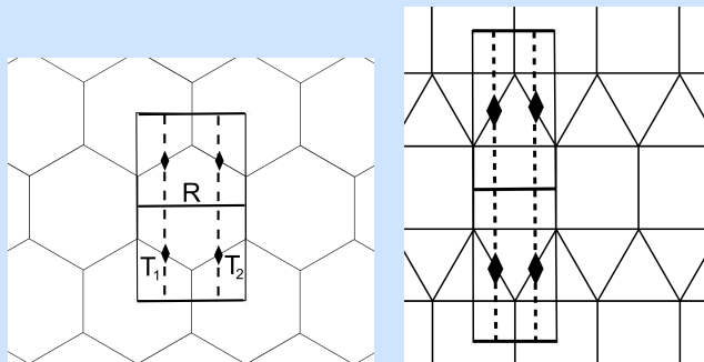
(b) Hexagonal tiling
