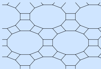
(h) Great rhombitrihexagonal tiling t_{\mathcal{T}} = 12
