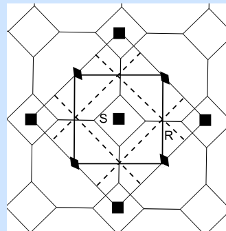
(b) p4g acting on the truncated square tiling
