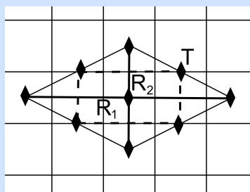
(a) Square tiling
