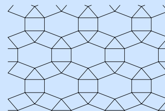
(f) Small rhombitrihexagonal tiling t_{\mathcal{T}} = 6
