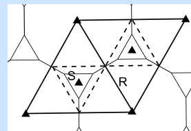
(b) Truncated hexagonal tiling
