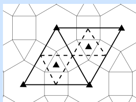
(a) Small rhombitrihexagonal tiling
