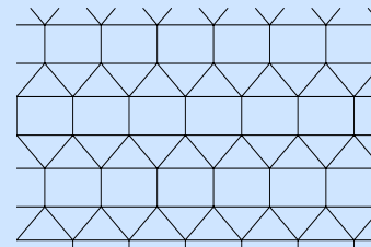
(l) Elongated triangular tiling t_{\mathcal{T}} = 2
