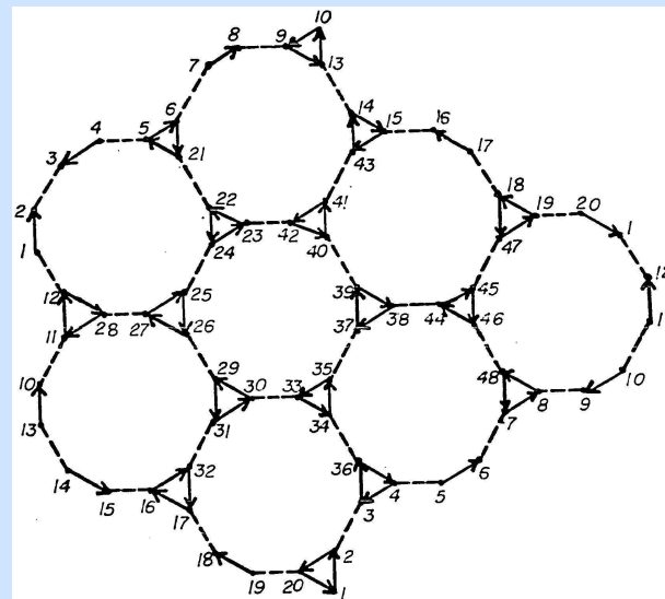
(b) Cayley graph for G_2
