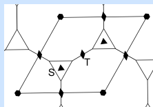
(b) Truncated hexagonal tiling
