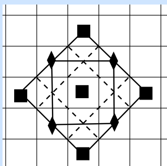
(a) p4g acting on the square tiling
