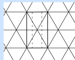
(b) Triangular tiling
