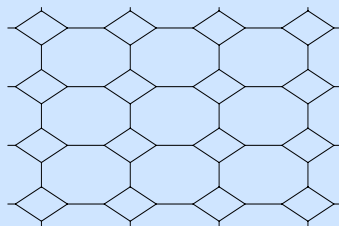
(j) Truncated square tiling t_{\mathcal{T}} = 4
