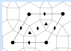
(a) Small rhombitrihexagonal tiling
