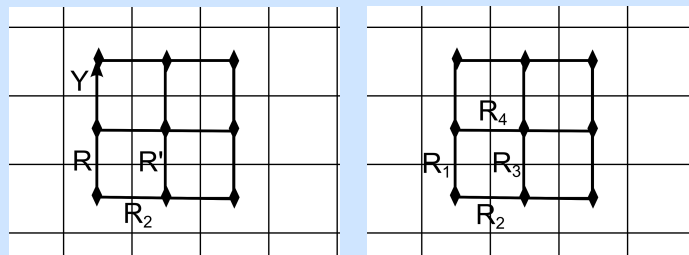
(a) Square tiling
