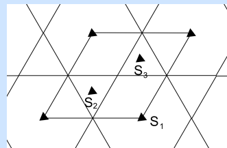
(b) Trihexagonal tiling
