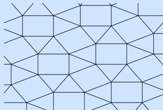
(k) Snub square tiling t_{\mathcal{T}} = 4
