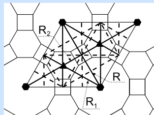
Figure 18. An FVT action of p6m on the great rhombitrihexagonal tiling.
