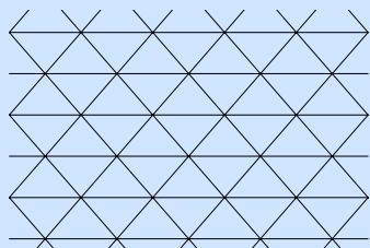
(a) Triangular tiling t_{\mathcal{T}} = 1
