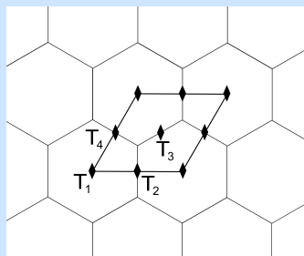
(c) Hexagonal tiling
