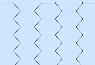
(b) Hexagonal tiling t_{\mathcal{T}} = 2
