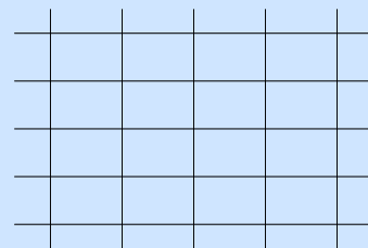
(i) Square tiling t_{\mathcal{T}} = 1
