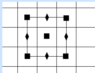
(a) Square tiling
