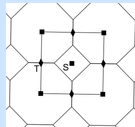
(c) Truncated square tiling
