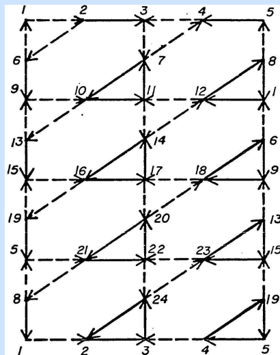
(a) Cayley graph for G_1
