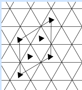
(a) Triangular tiling
