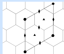
(c) Hexagonal tiling
