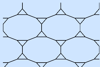
(g) Truncated hexagonal tiling t_{\mathcal{T}} = 6
