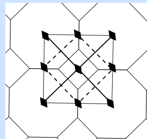
(b) Truncated square tiling
