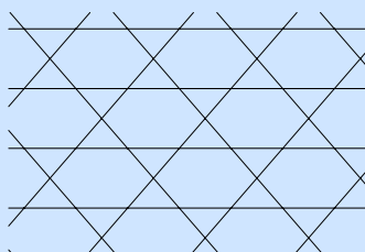
(e) Trihexagonal tiling t_{\mathcal{T}} = 3
