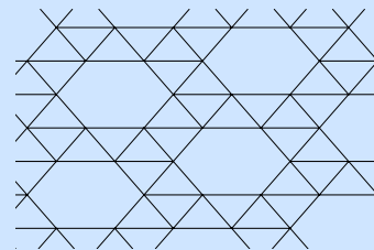
(c) Snub hexagonal tiling t_{\mathcal{T}} = 6
