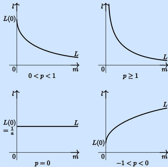
Figure 2. The relation between m = u(0) and l for u \in \mathcal{S}(l) in case II ( p > -1 , q = 0 , a > 0 ) according to Lemmata 2.8, 5.2 and 5.3. See also Theorem 5.4.
