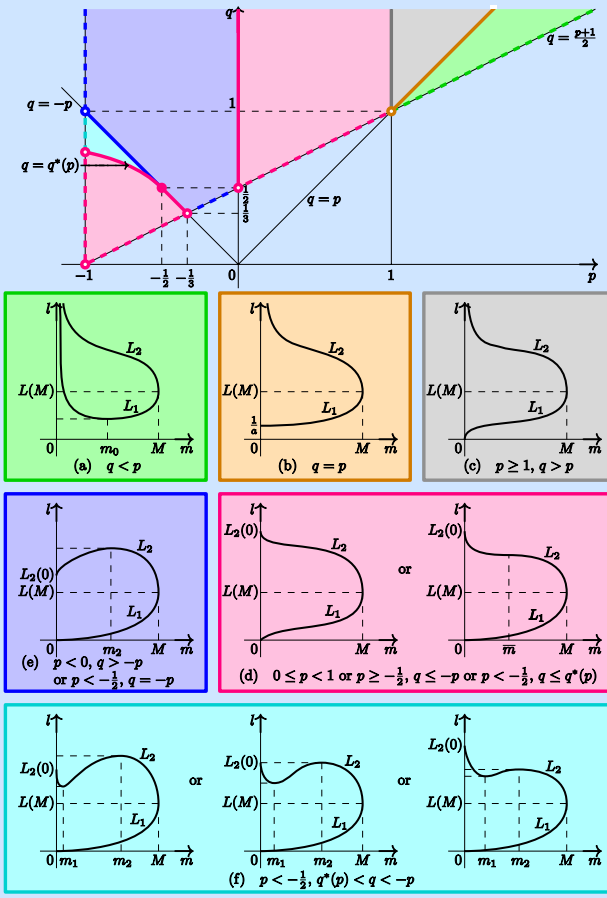
Figure 4. The relation between m = u(0) and l for u \in S(l) in case V ( p > -1, q > \frac{p+1}{2}, a > 0 ) according to Lemmata 2.8, 8.3, 8.4, 8.6, 8.7 and 8.8. See also Theorem 8.9.
