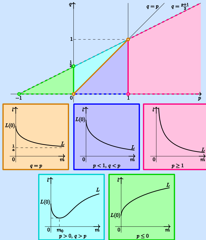
Figure 3. The relation between m = u(0) and l for u \in S(l) in case III ( p > -1 , 0 < q < \frac{p+1}{2} , a > 0 ) according to Lemmata 2.8, 6.2, 6.3, 6.4 and 6.5. See also Theorem 6.6.
