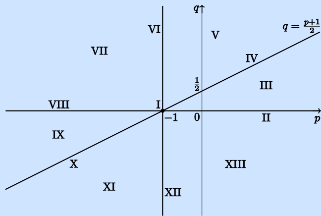
Figure 1. Cases I to XIII.
