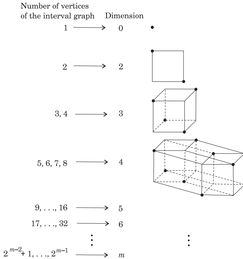
Figure 4. Number of 0-dimensional maximal intervals in the cubes of particular dimensions.
