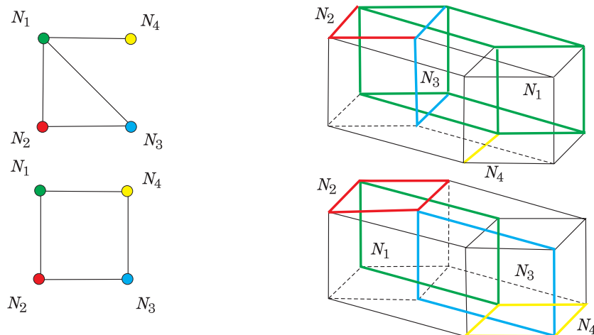
Figure 3. Graph G = (V, E) with |V| = 4 and |E| = 4 .
