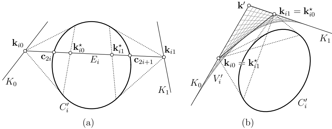
Figure 1. The construction of the points \mathbf{k}_{ij} and \mathbf{k}_{ij}^* (a) and its singularities (b).
