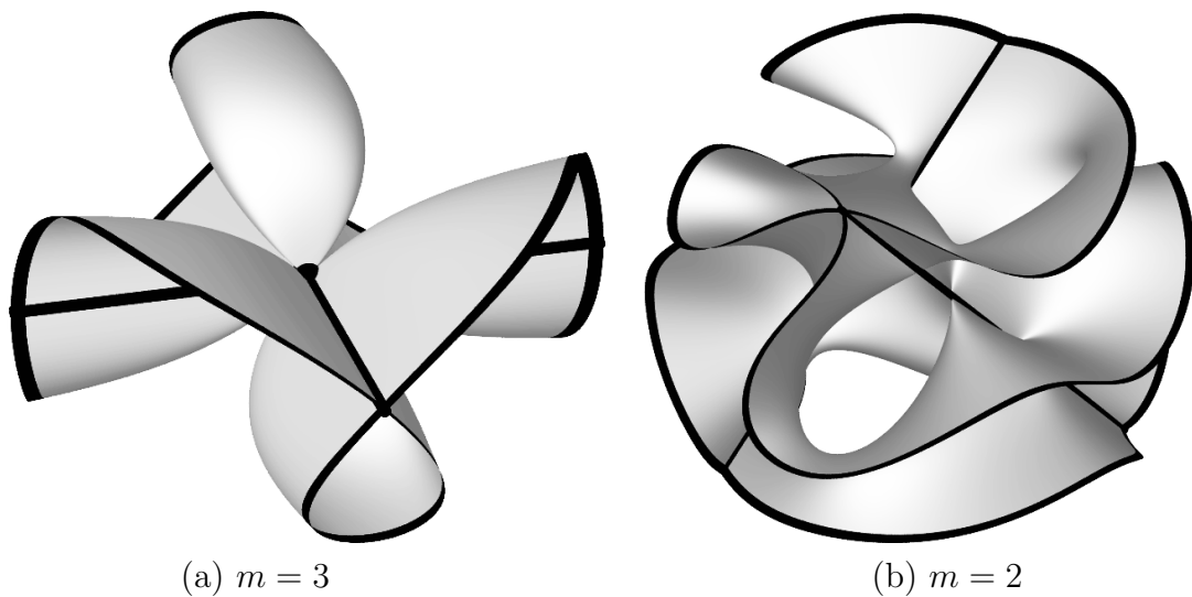
Figure 2. Dual solution surfaces
