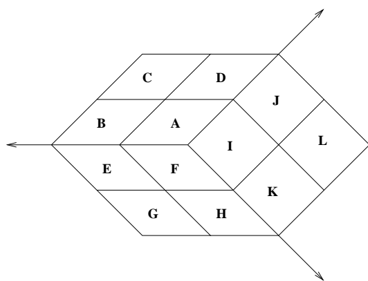
Figure 4: 1-dimensional branching
