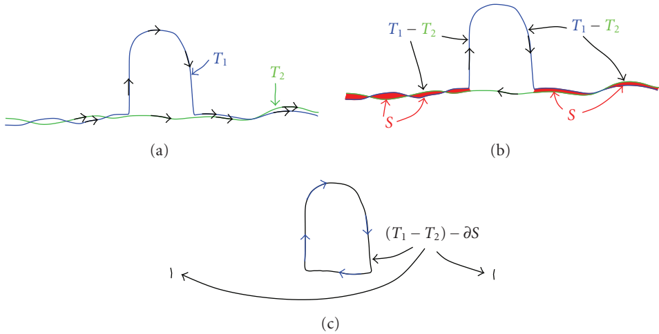
Figure A.4. The flat norm of the difference between these two currents is the sum of the area of red region ( L^1 like) and the length of the loop that is left.
