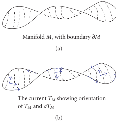
Figure A.1. Example 2-current T_M . Notice that \partial T_M = T_{\partial M} . The orientation on the boundary \partial M is simply that inherited from the orientation on M .
