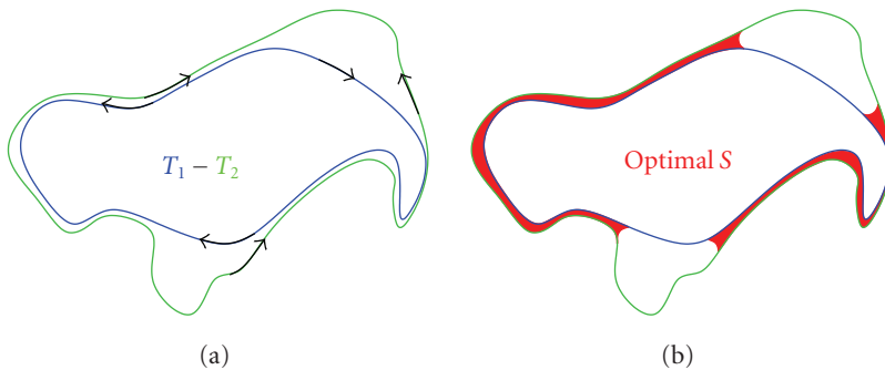
Figure 3.7. The flat norm via the L^1 TV functional provides us with both a distance and an informative optimal decomposition into S and T_1 - T_2 - \partial S . To use L^1 TV on sets, we need that T_1 = \partial\Omega_1 and T_2 = \partial\Omega_2 and either \Omega_1 \subset \Omega_2 or \Omega_2 \subset \Omega_1 . Using a direct method for computing the \mathbb{F}_\lambda we do not need these inclusions. Alternatively, we can identify the difference between two shapes \partial\Omega_1 and \partial\Omega_2 as the boundary of the set \Omega_1 \triangle \Omega_2 . Then we can use L^1 TV for all codimension 1, boundary shape differences, without requiring inclusions.
