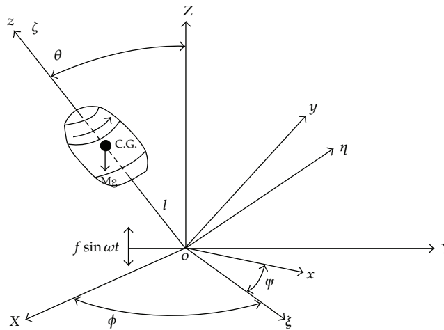
Figure 4: A schematic diagram of a symmetric gyroscope.
