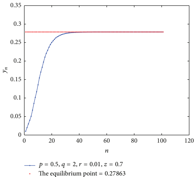
FIGURE 2: Dynamics of y_{n+1} = (0.01 + 0.5y_n + y_{n-3})/(0.7 + 2y_n + y_{n-3}) .
