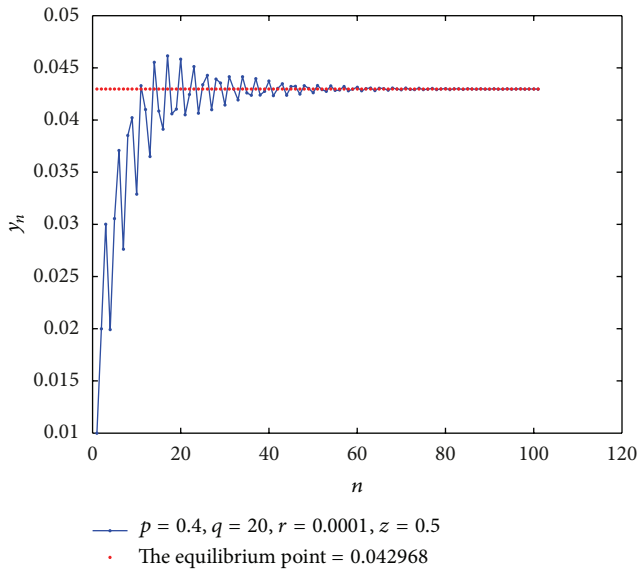
FIGURE 1: Dynamics of y_{n+1} = (0.0001 + 0.4y_n + y_{n-2})/(0.5 + 20y_n + y_{n-2}) .
