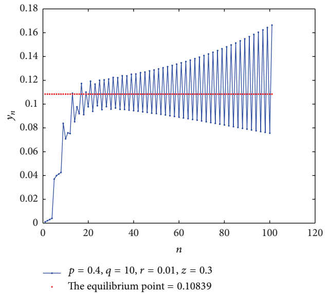
FIGURE 3: Dynamics of y_{n+1} = (0.01 + 0.4y_n + y_{n-3})/(0.3 + 10y_n + y_{n-3}) .
