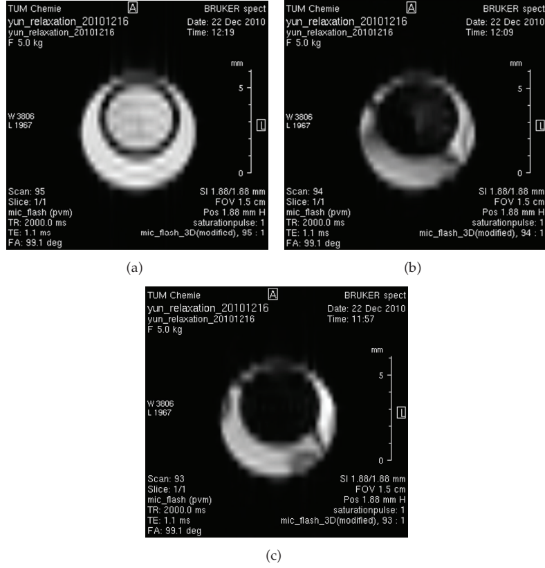
Figure 12: Experimental results on the contrast problems. The inner disk mimics the spin 1, while the outside ring mimics the spin 2. The two surfaces are separated by a thin black circle. (a) is a reference image before the application of the control field when the two spins are at the north pole of the Bloch sphere. (b) represent the contrast after a real experiment. The panel (b) corresponds to |M_y| , while the panel (c) to |M_z| , that is, the remaining y and z magnetization components after the optimized pulse. A color has been associated to each value of the contrast between 0 and 1, 0 and 1 corresponding, respectively, to the colors black and white. In the experiment, relaxation parameters are taken to be T_1 = 1.3 ms, T_2 = 50 ms for the inner sample and T_1 = 1.3 ms, T_2 = 200 ms for the outside sample.
