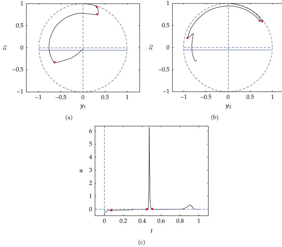
Figure 8: Trajectories of the magnetization vector for the first and second spins for the control field represented in the bottom panel. This field is the solution of the homotopy problem for \lambda = 0.93 . The red points indicate the possible structure of the solution in terms of bang and singular extremals (see the text).
