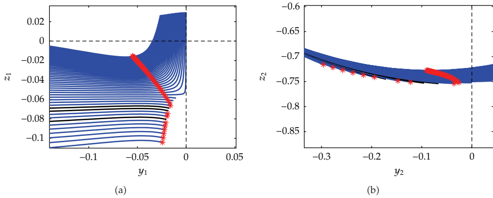
Figure 6: Zoom of the results of Figure 5.
