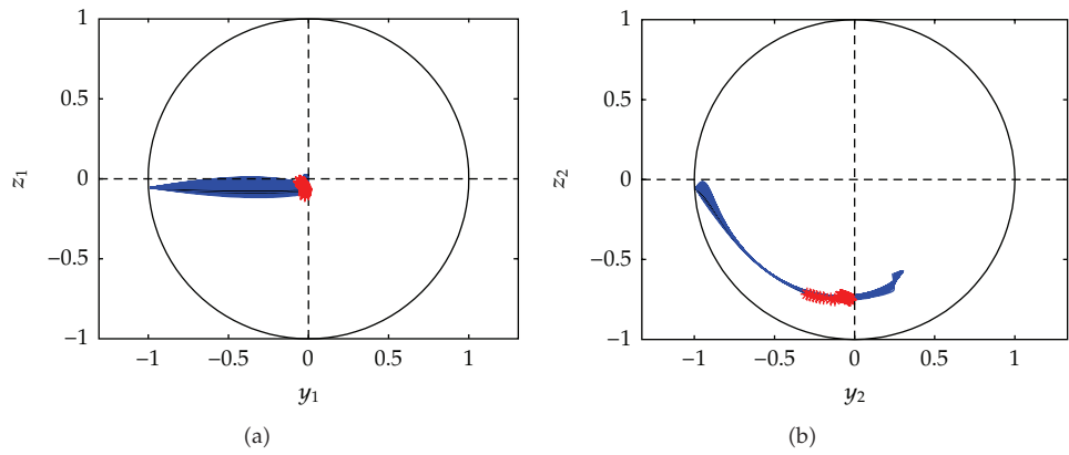
Figure 5: It is the same as Figure 3, but the conjugate points are computed along the singular extremals. Their positions are represented by red crosses.
