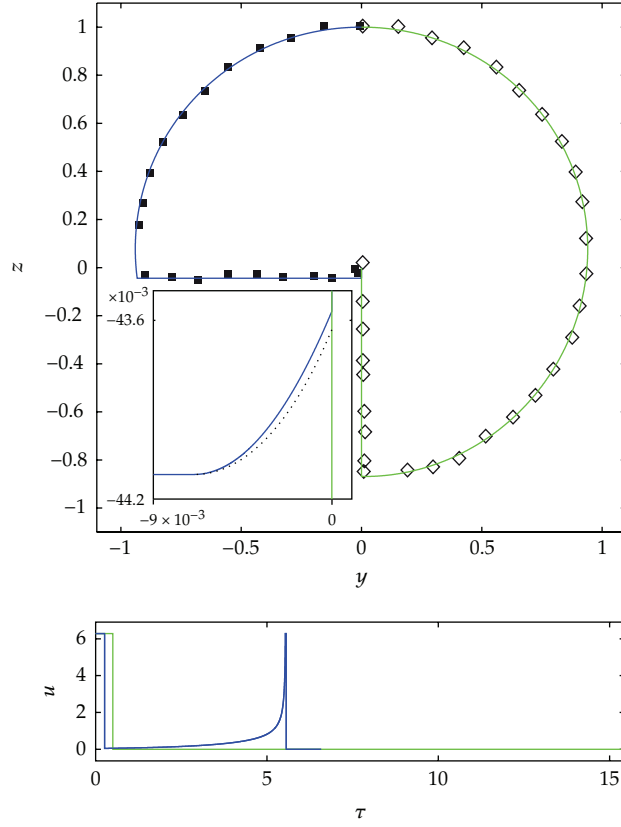
Figure 2: Plot of the optimal trajectories (left) and of the inversion recovery sequence (right) in the plane (y, z) . Experimental parameters are taken to be T_1 = 740 ms, T_2 = 60 ms, and \omega_{\max}/(2\pi) = 32.3 Hz. The experimentally measured trajectories are represented by filled squares and open diamonds. In the upper panel, the small insert represents a zoom of the optimal trajectory near the origin. The dotted line is the switching curve originating from the horizontal singular line. The solid curve is the optimal trajectory near the origin. The lower panel displays the corresponding control laws. \tau is the reduced time defined by \tau = (\omega_{\max}/(2\pi))t .
