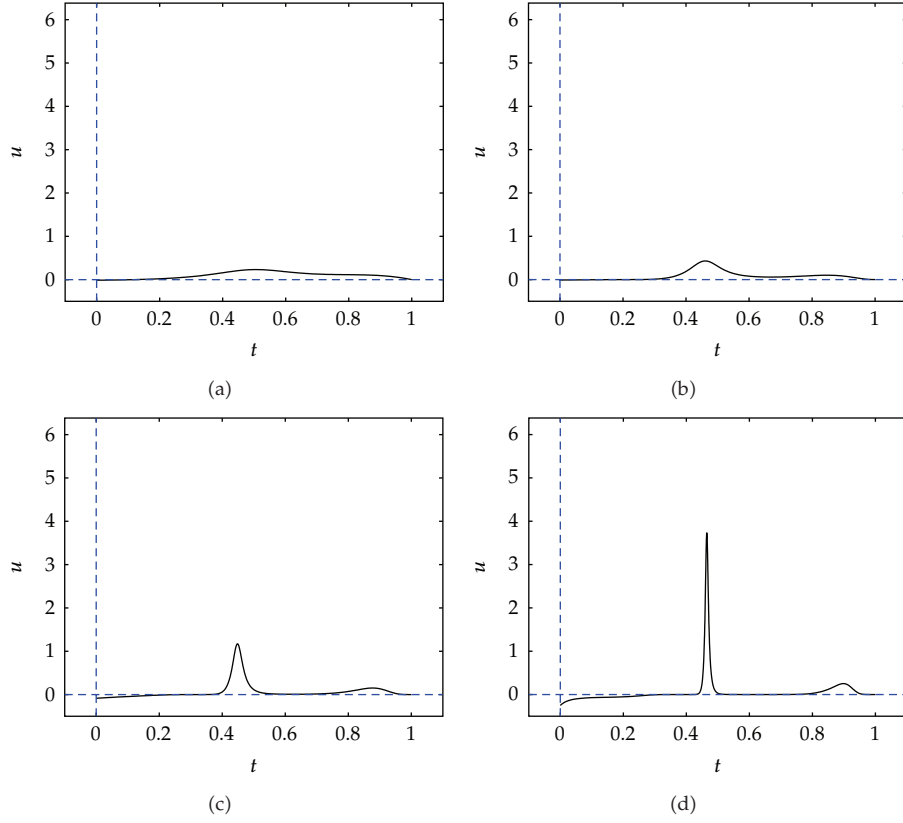
Figure 7: Evolution of the control field u for different values of the homotopy parameter \lambda , which is equal to 0, 0.6, 0.8, 0.9 from (a) to (d). The transfer time normalized to 1 is equal to 2T_{\min} .
