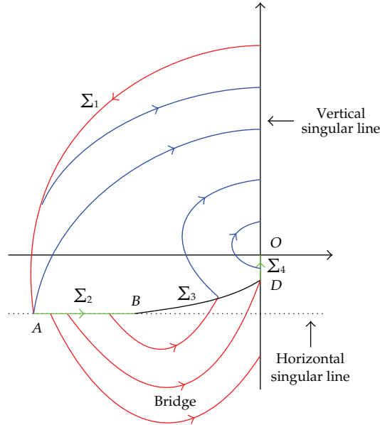
Figure 1: Global synthesis from the north pole. The switching locus \Sigma is formed by the union of the surfaces \Sigma_i . Due to the symmetry of revolution, the cut locus corresponds to the z -axis.
