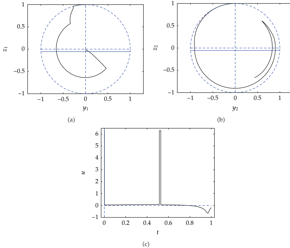
Figure 9: It is the same as Figure 8, but for a control field with a BSBS structure. Note the similarity of this result with the one of Figure 8.
