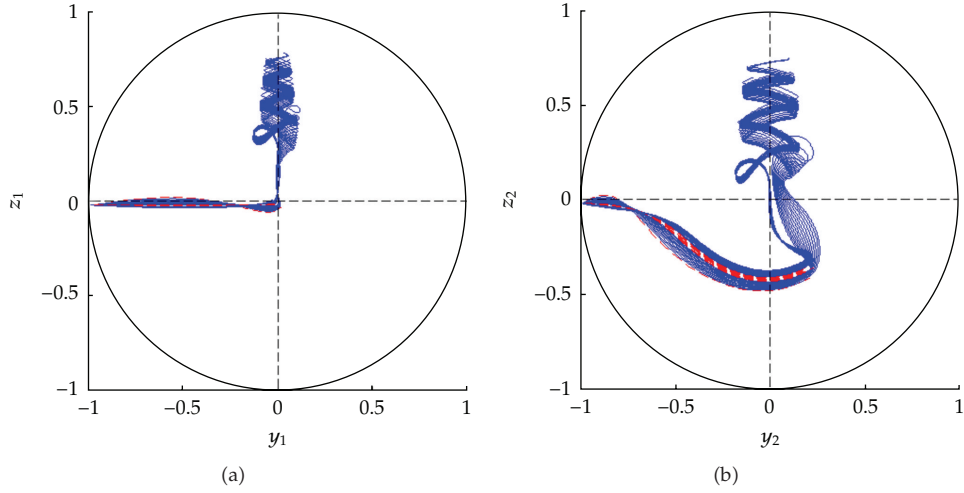
Figure 4: It is the same as Figure 3, but the singular flow is followed for longer times to show the attracting property of the north pole for the singular flow.
