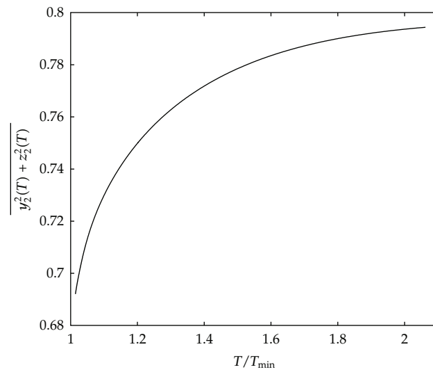
Figure 11: Evolution of the final contrast as a function of the transfer time.
