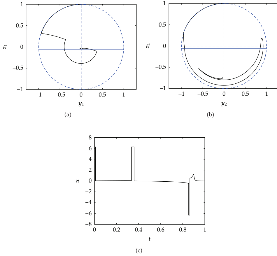
Figure 10: It is the same as Figure 9 but for a control field of the form BSBSBS with t_f = 1.1T_{\min} .
