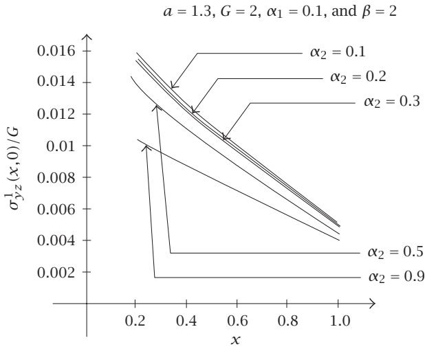
FIGURE 3.4. Variation of \sigma_{yz}^1(x,0)/G_1 with x for different values of \alpha_2 = 0.1, 0.3, 0.5, 0.7, 0.9 , a = 1.3 , G = 2 , \alpha_1 = 0.1 , and \beta = 2 .
