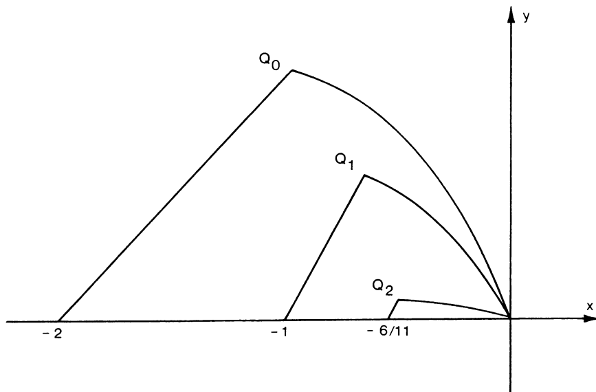
Fig. 1. Stability regions for Adams-Bashforth methods for k=0,1,2 .
