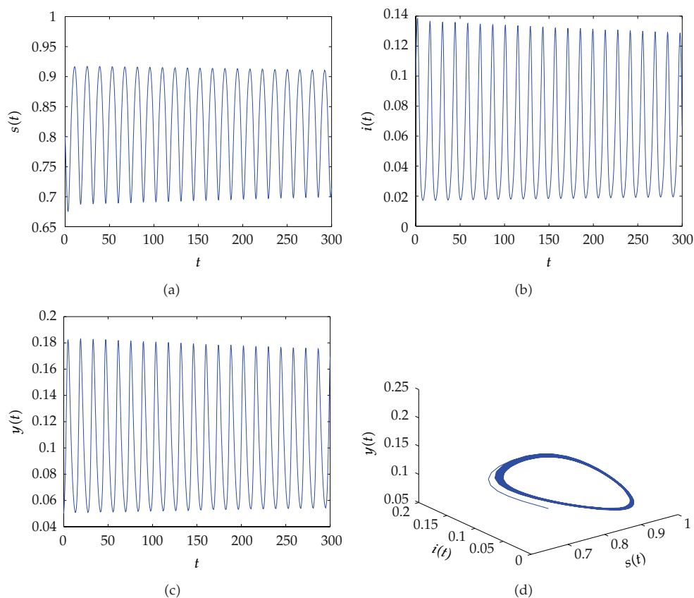
Figure 2: Trajectory portrait and phase portrait of system (3.1) with \tau_1 = 0 , \tau_2 = 0.415 > \tau_{20} \approx 0.32 . Hopf bifurcation occurs from the positive equilibrium E_0(0.82, 0.06, 0.1033) . The initial value is (0.8, 0.1, 0.05) .
