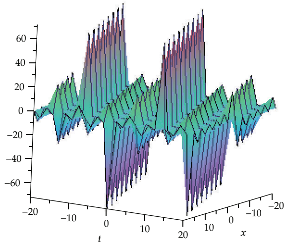
Figure 8: Solitons solution for \lambda = 1, \mu = 1 .
