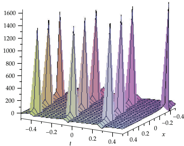
Figure 9: Solitons solution for \lambda = 7, \mu = 14 .
