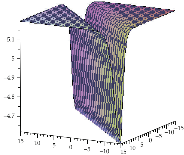
Figure 6: Periodic solution for \lambda = 3, \mu = 2 .
