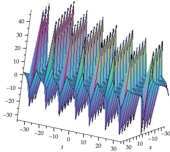
Figure 10: Solitons solution for \lambda = 6, \mu = 10 .
