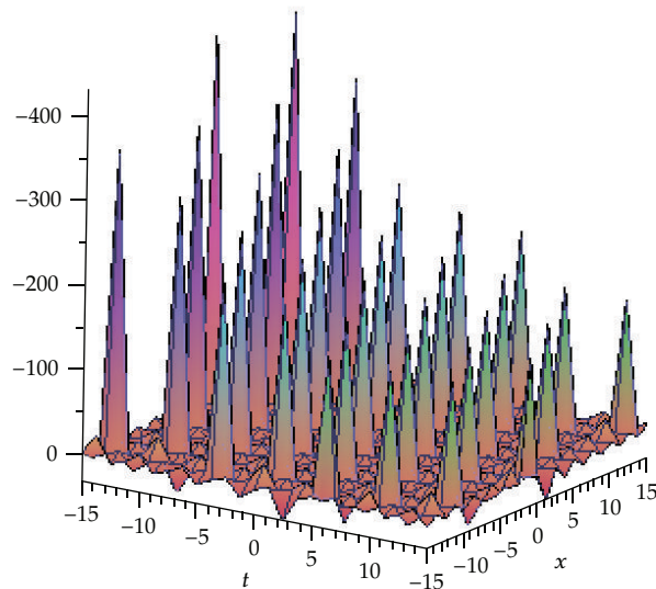
Figure 13: Solitons solution for \lambda = 3, \mu = 4 .
