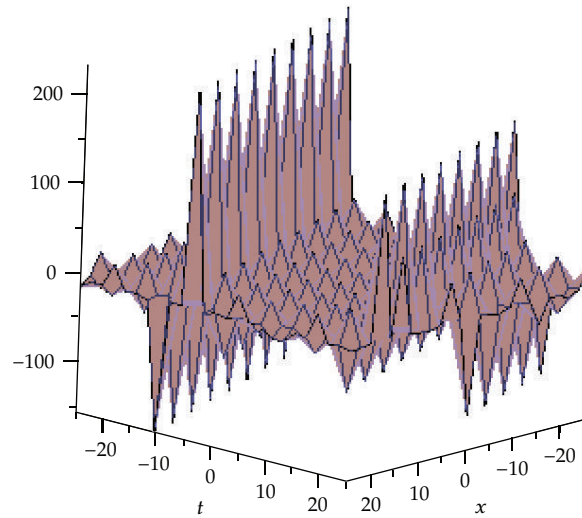
Figure 12: Solitons solution for \lambda = 3, \mu = 3 .
