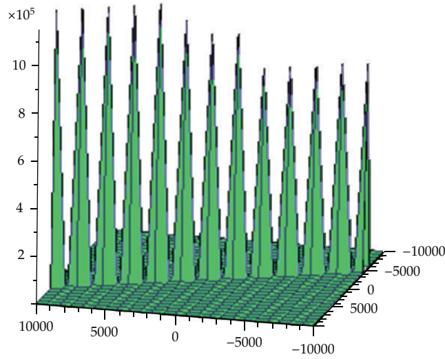
Figure 2: Solitons solution for \lambda = 2, \mu = 0.5 .
