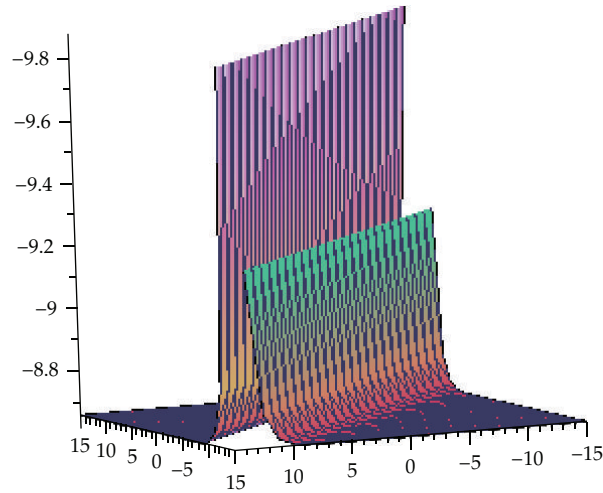
Figure 4: Periodic solution for \lambda = 5, \mu = 6 .
