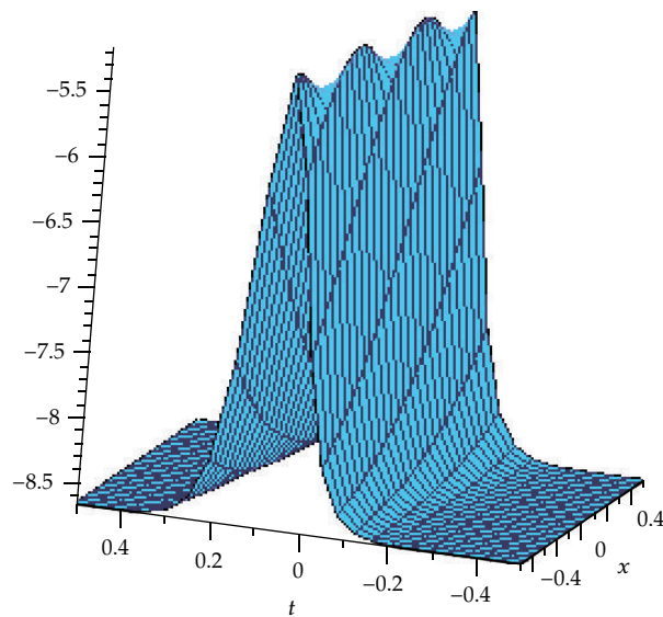
Figure 5: Periodic solution for \lambda = 5, \mu = 4 .
