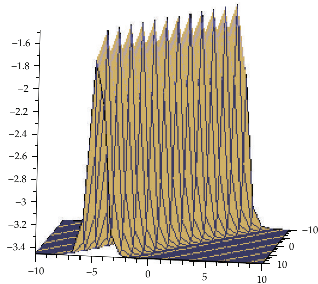
Figure 7: Solitons solution for \lambda = 2, \mu = 0.5 .
