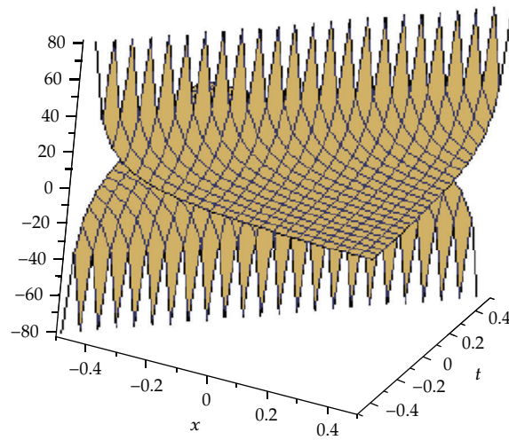
Figure 1: Solitons solution for \lambda = 3, \mu = 2 .
