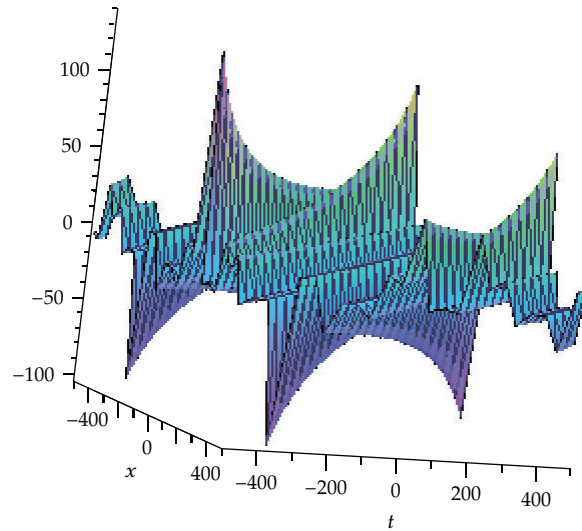
Figure 14: Periodic solution for \lambda = 0.5, \mu = 1 .
