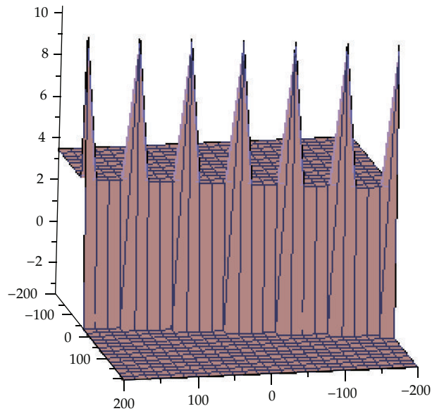
Figure 3: Solitons solution for \lambda = 6, \mu = 8 .
