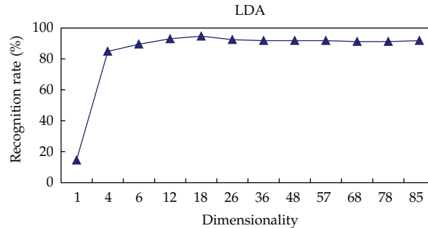
Figure 7: LDA recognition performance according to dimensionality via LDA algorithm with nearest neighbor classifier.
