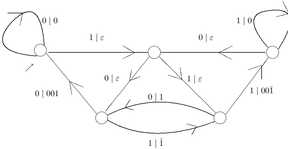
Figure 3: The binary \rightarrow “ 1 = 5/4 - 1/4 ” transducer
