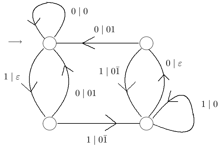
Figure 1: The binary \rightarrow Paul transducer
