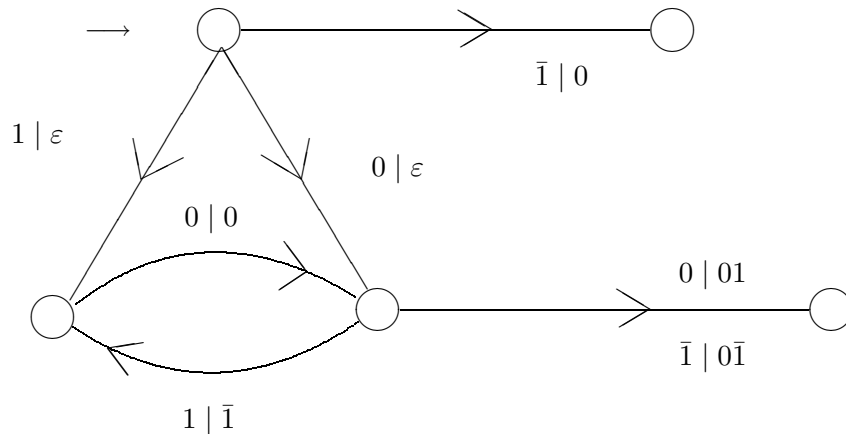
Figure 2: Adding 1 in the Paul representation
