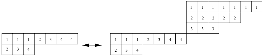
Fig. 5 An instance of the correspondence between \mathbb{T}(\lambda, \mu) and \text{LR}\mathbb{T}(\lambda * \alpha, \nu) for \lambda = (7, 3) and \mu = (3, 2, 2, 3) , \alpha = (7, 5, 3) and \nu = (10, 7, 5, 3)
