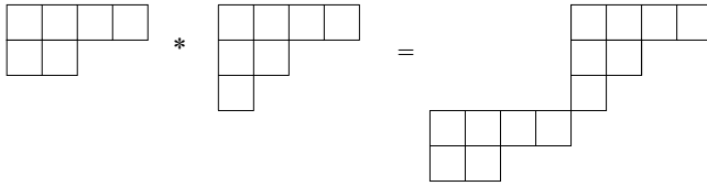
Fig. 1 Left to right, the shapes \lambda , \alpha and the skew shape \lambda * \alpha
