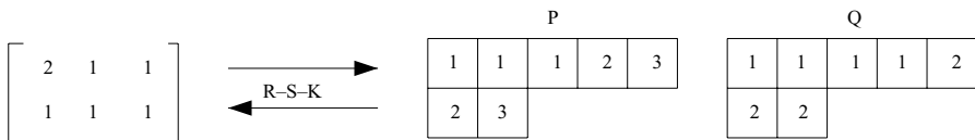
Fig. 2 An instance of the correspondence between \mathbb{I}(\mathbf{a}, \mathbf{b}) and \cup_{\check{\lambda}} \mathbb{T}(\check{\lambda}, \mathbf{a}) \times \mathbb{T}(\check{\lambda}, \mathbf{b}) for \mathbf{a} = (4, 3) , \mathbf{b} = (3, 2, 2)
