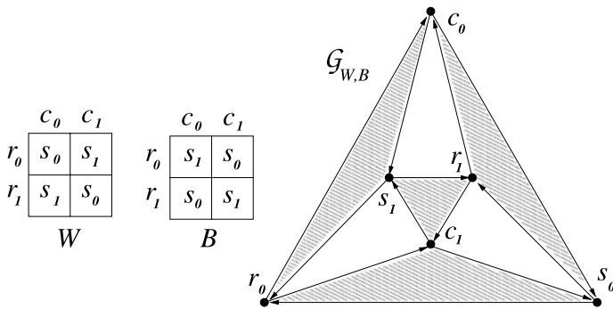
Fig. 1 Intercalates (W, B) with the corresponding triangulation \mathcal{G}_{W,B}
