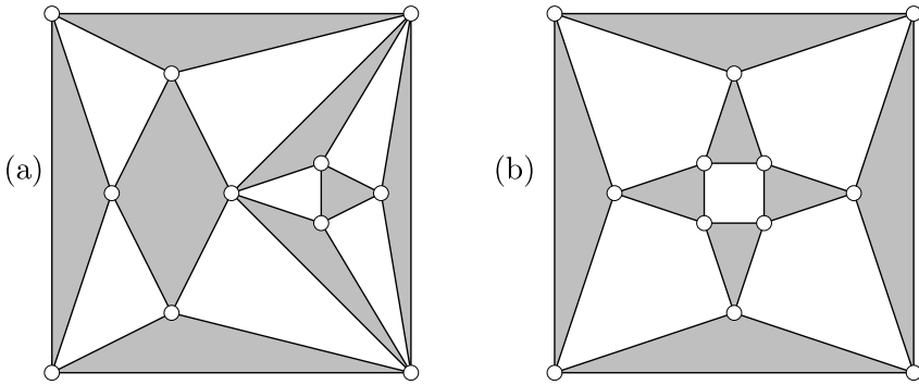
Fig. 3 Two face 2-colourable plane graphs
