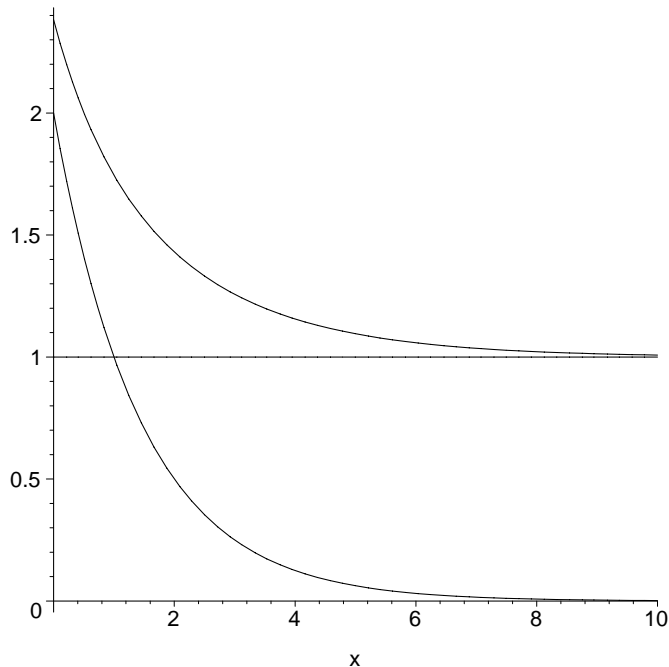
Figure 6: Diagram, from top to bottom, of \theta(\lambda^*, x) , 1 and 2^{-(x-1)} where \lambda^* satisfies (4.9) – (4.10).
