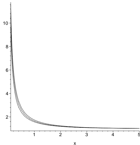
Figure 7: Plot of m(x) = \max \{L(x), L_2^*(x)\} , \zeta(x+1) and M(x) = \min \{U^*(x), U_2(x)\} where L(x) , L_2^*(x) , U^*(x) and U_2(x) are defined by (2.18), (4.13), (4.11) and (2.21) respectively.
