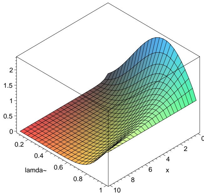
Figure 4: A plot of 4 \cdot \lambda^{x+1} , 0 < \lambda \leq \frac{1}{2} and \theta(\lambda, x) = \lambda^{x-1} \left( \frac{\lambda}{1-\lambda} \right)^{2(1-\lambda)} , \frac{1}{2} \leq \lambda < 1 .
