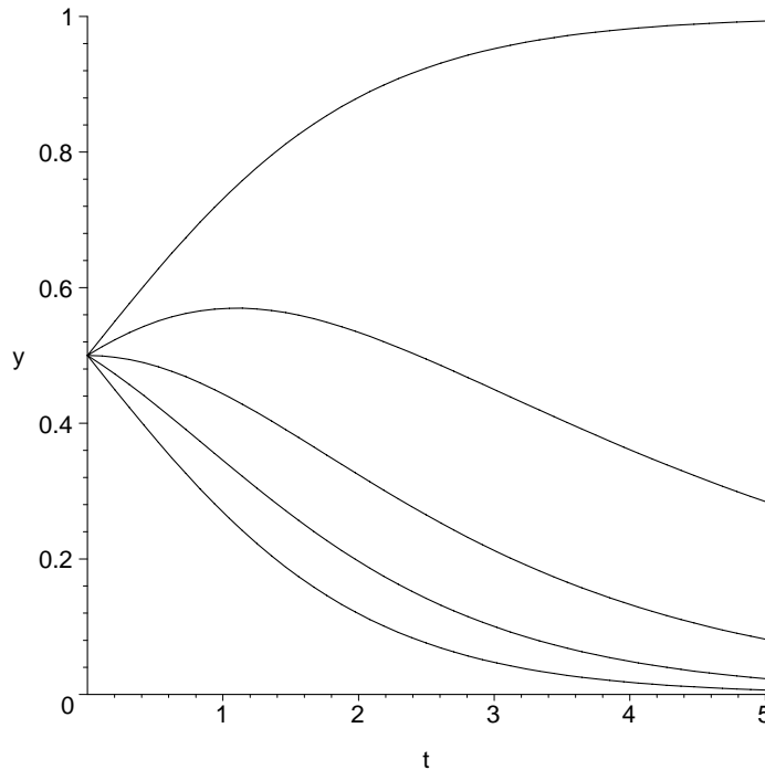
Figure 3: Plot of \frac{1}{h_\lambda(t)} for \lambda = 0, \frac{1}{4}, \frac{1}{2}, \frac{3}{4} and 1 in order from bottom to top. The lower bound H_\lambda(t) is zero for 0 \leq \lambda < 1 and \frac{e^{-\lambda t}}{2} for \lambda = 1 .
