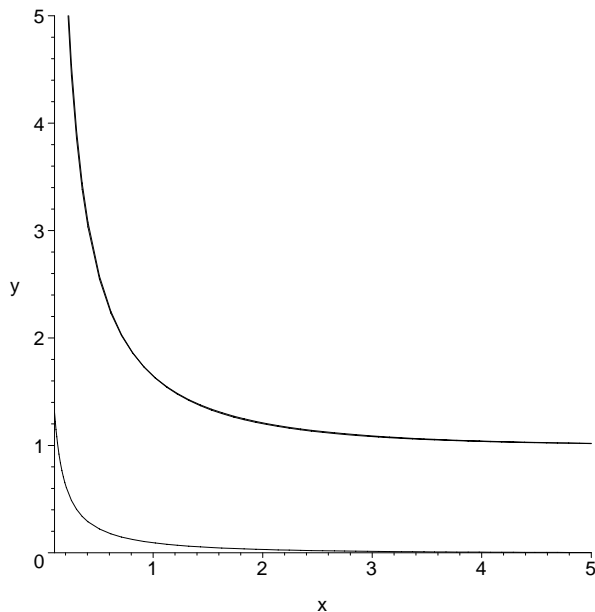
Figure 2: Plot of \zeta(x+1) , its approximation \frac{\zeta(x+2) - \frac{5}{16}b(x+1)}{1-b(x+1)} and its bound \frac{3}{16} \cdot \frac{b(x+1)}{1-b(x+1)} where b(x) is as given by (2.9). This represents the implementation of Corollary 2.5.
