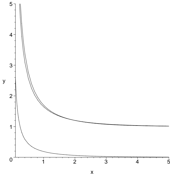
Figure 1: Plot of \zeta(x+1) , its approximation (1 - b(x))\zeta(x) + \frac{5}{16}b(x) and error bound \frac{3}{16}b(x) where b(x) is as given by (2.9). This represents the implementation of Corollary 2.3.
