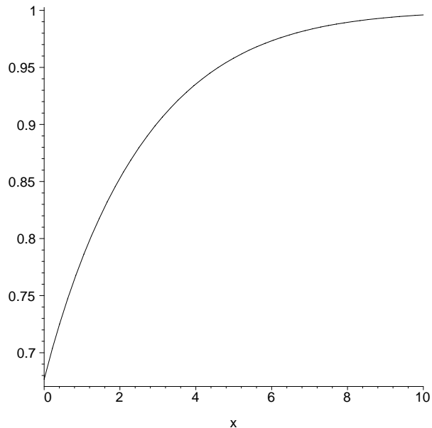
Figure 5: A plot of \lambda^* , satisfying (4.9) – (4.10) which produces \max_{\lambda \in [\frac{1}{2}, 1)} \theta(\lambda, x) = \theta(\lambda^*, x) .
