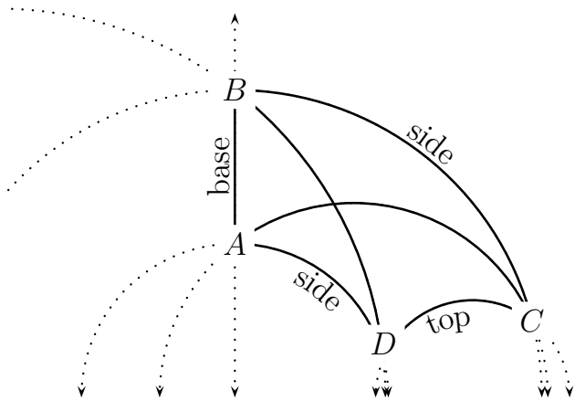
Figure 3: A Saccheri quadrilateral: \angle A = \angle B = \pi/2 and \angle C = \angle D , whence AD = BC and AC = BD
