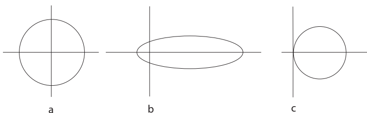
FIGURE 1. Three possibilities for an isoperimetric region in the plane with density r^p , p > 0 . The first circle (a) is unstable, the last circle (c) is the minimizer.
