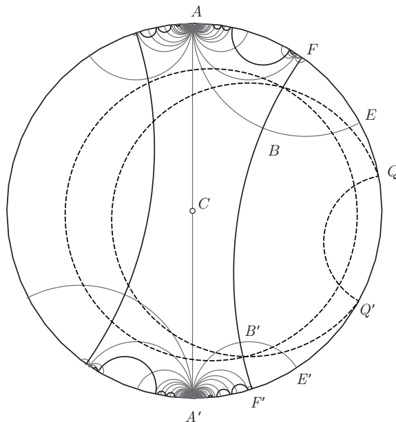
FIGURE 3. An ample cone \mathcal{K} intersected with \mathcal{H} , the region bounded by the dark lines. The gray lines represent the symmetries of \mathcal{K} \cap \mathcal{H} , or the tiling of \mathcal{K} \cap \mathcal{H} with \mathcal{F}' . The dotted curves represent the line P \circ \mathbf{x} = 0 , the curve -P \circ \mathbf{x} = t , and a disc that contains the intersection of \mathcal{K} \cap \mathcal{H} with the region -P \circ \mathbf{x} \leq t .
