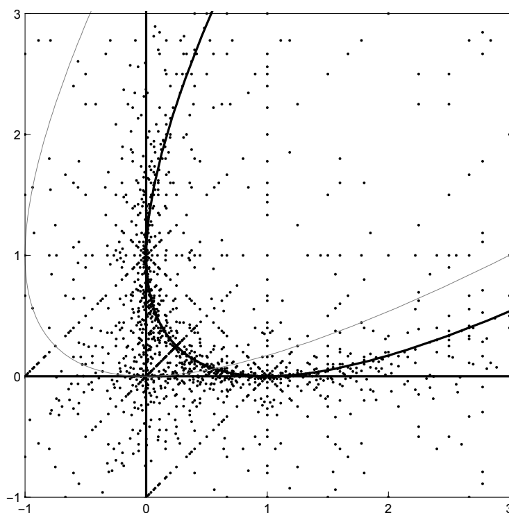
FIGURE 6.1. A window on U_{2,1,1,1}(\mathbb{R}) , which is the complement of the three thick discriminantal curves in the u - v plane. Points are part of the specialization set U_{2,1,1,1}(\mathbb{Z}[1/30]) which is used in both §6 and §9. The thin parabola (u - v)^2 = 4v plays a role only in §6.
