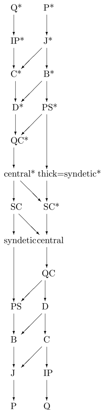
Figure 1: Implications for S = \mathbb{N}^v or \mathbb{Z}^v .
