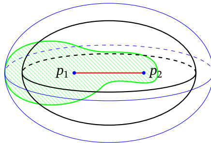
FIGURE 6. Barriers used in Theorem 4.19.
