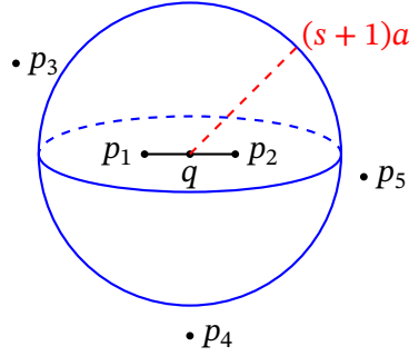
FIGURE 8. Example of distribution of points satisfying the condition given in Proposition 1.7.
