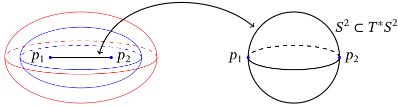
FIGURE 2. Equivalence of Eguchi–Hanson metric to two centre Gibbons–Hawking metric.
