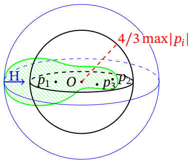
FIGURE 4. Spherical barriers used in Theorem 4.5.
