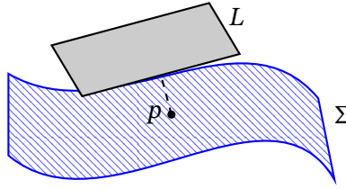
FIGURE 1. Plane that violates convexity in Proposition 3.19.
