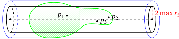
FIGURE 5. Cylindrical barriers used in Theorem 4.7.
