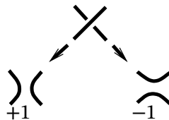
FIGURE 1. Positive and Negative Smoothings
