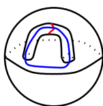
FIGURE 5. A trivial handle with standard meridians shown in red and blue
