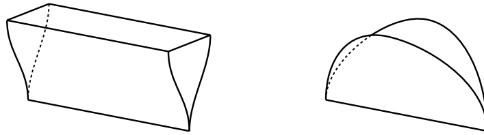
FIGURE 25. Forgetting the corner structure of a 1-cusped triangle times interval (left) results in a taco (right).
