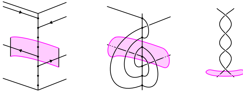
FIGURE 15. Performing halved \frac{1}{-k} horizontal surgery on an annulus around a cone point adds k half twists to the corresponding rational tangle.
