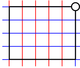
FIGURE 4. A perfect fit rectangle.
