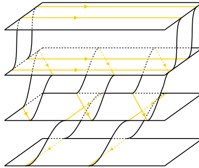
FIGURE 13. Rough picture of \widetilde{B}_0 .
