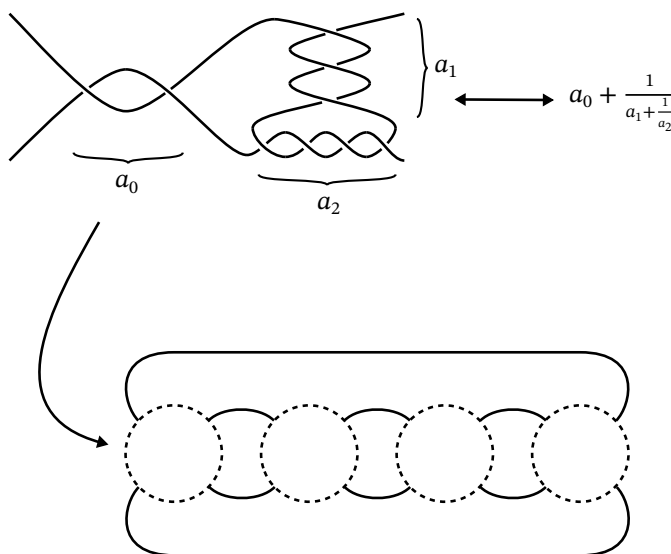
FIGURE 5. Definition of a Montesinos link.
