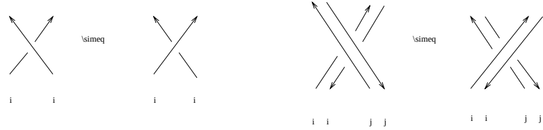
FIGURE 24. Two local moves that generate the relation of surgery equivalence. Here arcs labeled by the same letter ( i or j ) belong to the same link component.
