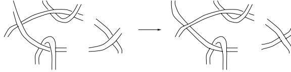
FIGURE 41. A double crossing change of bands in opposite directions.
