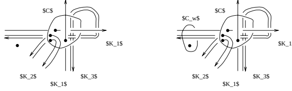
FIGURE 21. Shown here on the left-hand side are the 3 arcs along which a ball B intersects the knot K_1 , the 2 arcs along which it intersects K_2 and the 2 arcs that it intersects the knot K_3 . Shown also is an unknotted component C which bounds a disc D , and with bold dots are the points where D intersects K_1 and K_2 . On the right-hand side of the figure is shown one of the links (C_w) that appears in equation (17).
