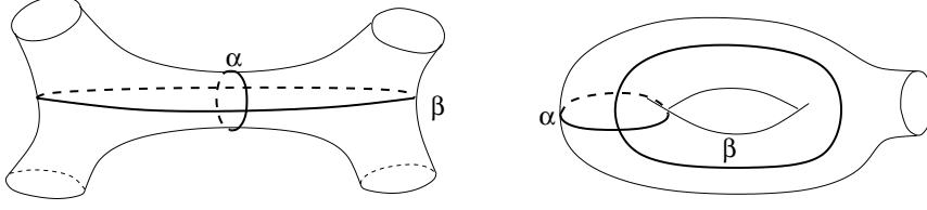
Figure 5: Pants decomposition
