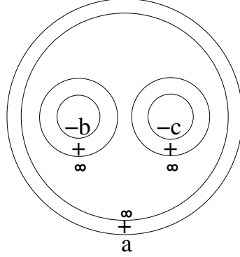
Figure 7: Factoring
