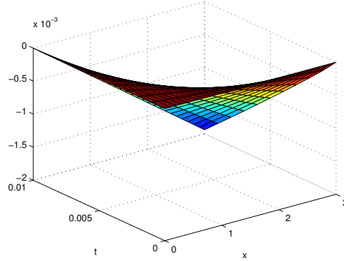
FIGURE 3. The solution of (4.3)
