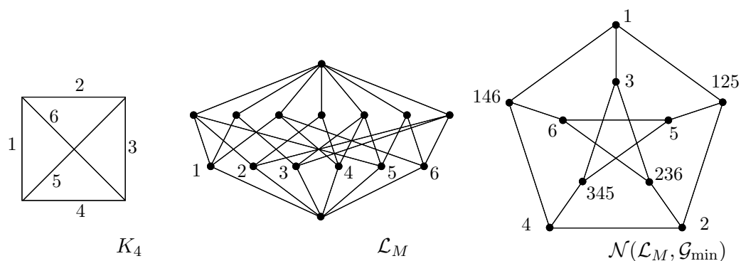
Figure 2 – The lattice of flats \mathcal{L}_M and its minimal nested set complex \mathcal{N}(\mathcal{L}_M, \mathcal{G}_{\min}) .
