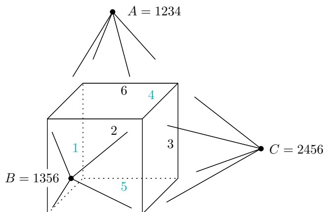
Figure 1 – The cube realization of M
