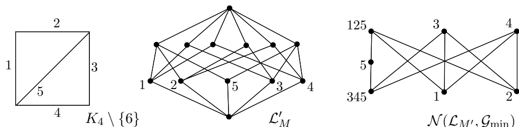
Figure 3 – The lattice of flats \mathcal{L}_{M'} and its nested set complex \mathcal{N}(\mathcal{L}_{M'}, \mathcal{G}_{\min}) .
