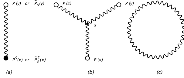
Figure 2. Preons are bound by hyper-magnetic strings: (a) corresponds to the “unclosed” string configurations of composite quark-leptons, hyper-gluons and hyper-Higgses; (b) corresponds to “baryonic” and “diquark” configurations; (c) represents a closed string describing a hyper-glueball (“graviton”).
