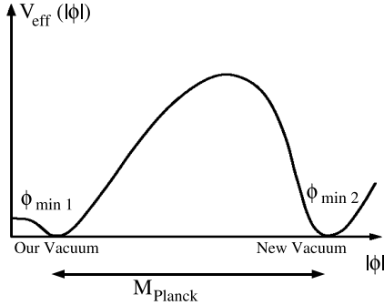
Figure 1. The first (our) vacuum at |\phi| \approx 246 GeV and the second vacuum at the fundamental scale |\phi| \sim M_{Pl} .
