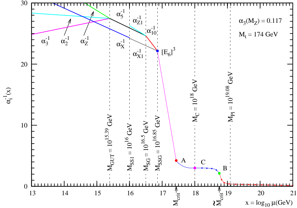
Figure 3. The figure provides a qualitative description of the running of \alpha^{-1}(x) near the Planck scale predicted by the present preon model. The family replicated gauge group of symmetry [E_6]^3 exists in the region of energies M_{SSG} \leq \mu \leq M_{\text{crit}} . The point A at the scale of energy \mu = M_{\text{crit}} indicates that hyper-electric preon strings exist for \mu \geq M_{\text{crit}} . The point B corresponds to the scale \mu = \widetilde{M}_{\text{crit}} and indicates that hyper-magnetic preon strings exist for \mu \leq \widetilde{M}_{\text{crit}} . The curve AB corresponds to the region of spreon condensation, where we have both hyper-electric and hyper-magnetic strings. The point C corresponds to the second vacuum of our theory. For \mu \geq \widetilde{M}_{\text{crit}} we have the running of \alpha^{-1}(x) for monopolic “quark-leptons”, but gravity (SUGRA) transforms the trans-Planckian region. We assume that our theory is valid only up to the scale \sim 10^{18} GeV (point C ).
