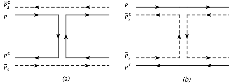
Figure 4. Vector gauge bosons belonging to the 78 representation of the flipped E_6 and Higgs scalars – singlets of E_6 – are composite objects created (a) by fermionic preons P , P^c and (b) by scalar spreons \tilde{P}_s , \tilde{P}_s^c . Both of them are confined by hyper-magnetic strings.
