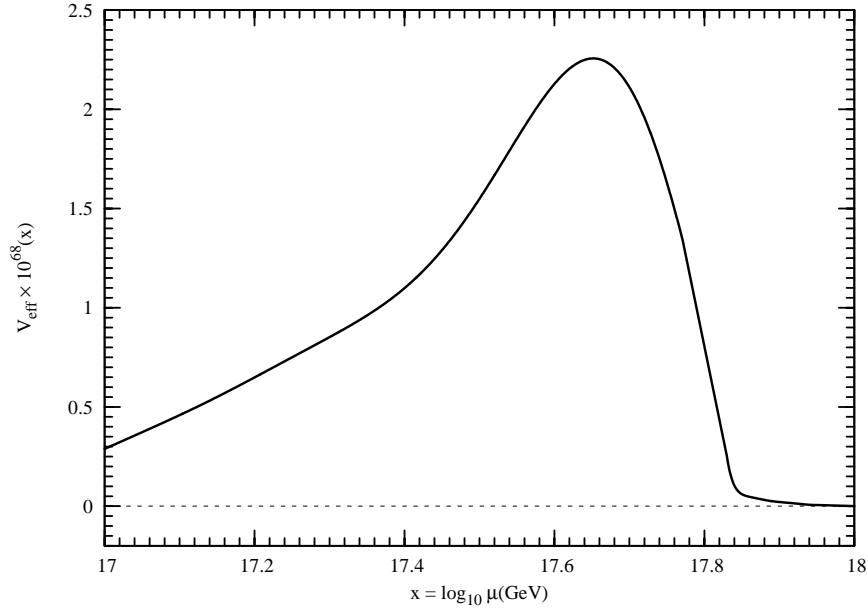
Figure 5. The behavior of the effective potential V_{\text{eff}}(x) for the E_6^3 theory, showing a second minimum of our theory at the point \mu = M_C = 10^{18} GeV. This minimum is given by the requirement: V_{\text{eff}} = V'_{\text{eff}} = 0 , according to the Multiple Point Principle.
