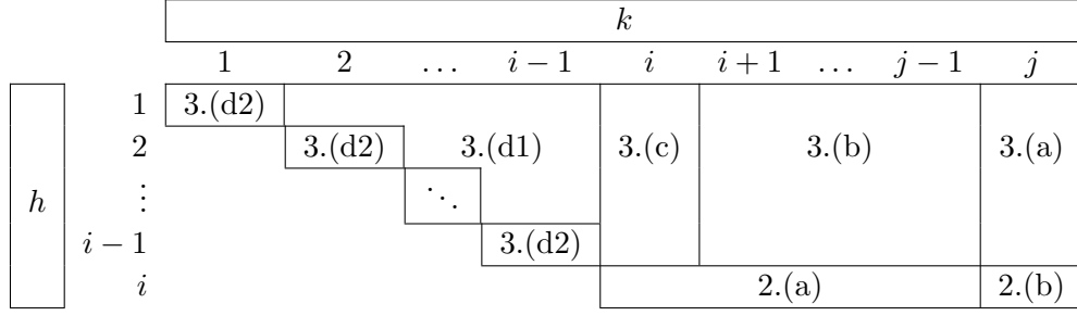
Figure 2. Possible combinations of h and k in the terms u_{hk}^\delta used as labels for columns in the contracted matrix. Each term u_{hk}^\delta corresponds to one subcase in the consideration of cases 2. h = i and 3. h < i . Each of these subcases refers to one of the terms in square brackets in Lemma 2 as follows: 2.(a) – line (17), 2.(b) – line (19), 3.(a) – line (18), 3.(b) – line (16), 3.(c) – line (15), 3.(d1) – line (14), 3.(d2) – line (13).
