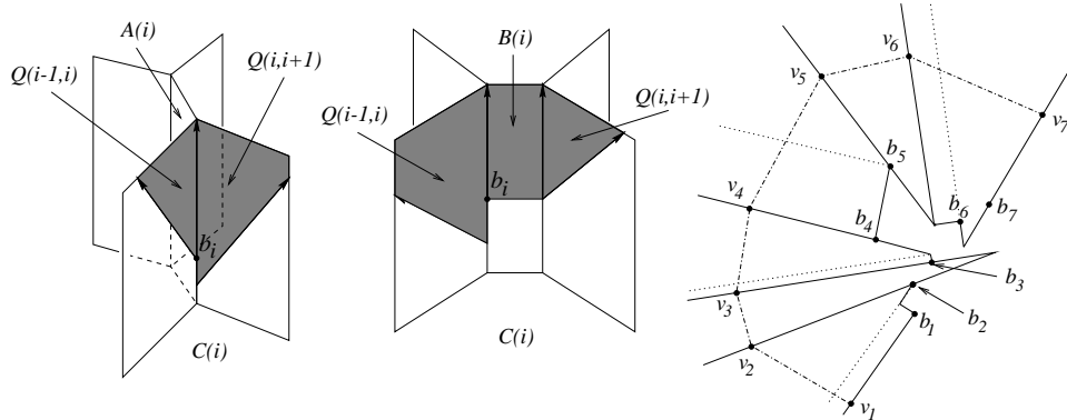
Figure 1: Examples of C(i) and the construction of the polygon P(v_1, \dots, v_m)
