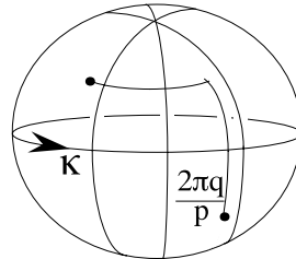
Figure 2: Standard spine of L(p, q) and core \kappa
