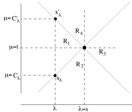
Figure 8: Configuration of (s, t) in \Gamma
