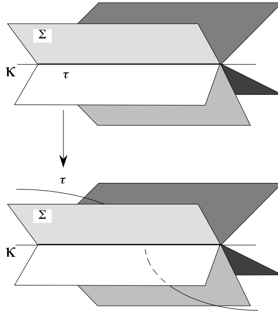
Figure 12: Isotopy of \tau with respect to the spinal helix
