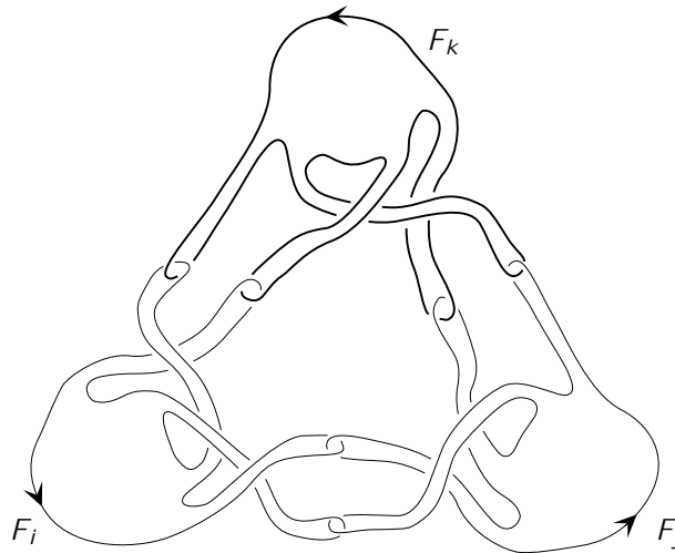
Figure 3: Disentangled surfaces
