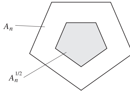
Figure 4: The small copy A_n^{1/2} does not touch any other A_n .
