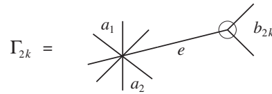
Figure 7: b_{2k} is left out.
