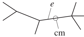
Figure 3: Center of mass (circle) for tree with 6 leaves
