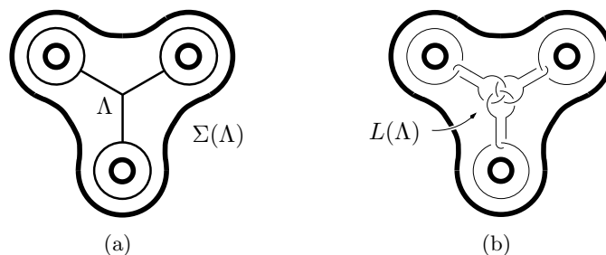
Figure 1: Y-graph and associated link
