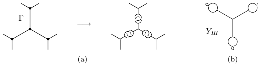
Figure 2: Turning a Jacobi diagram into a Y -link
