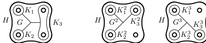
Figure 10: Splitting a leaf
