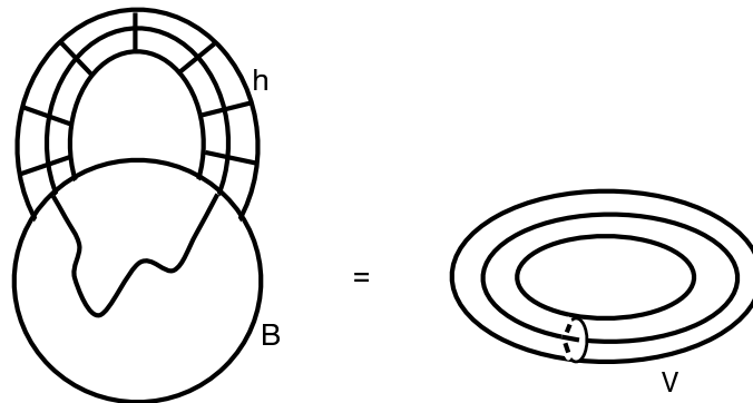
Figure 6: B \cup h seen as solid torus
