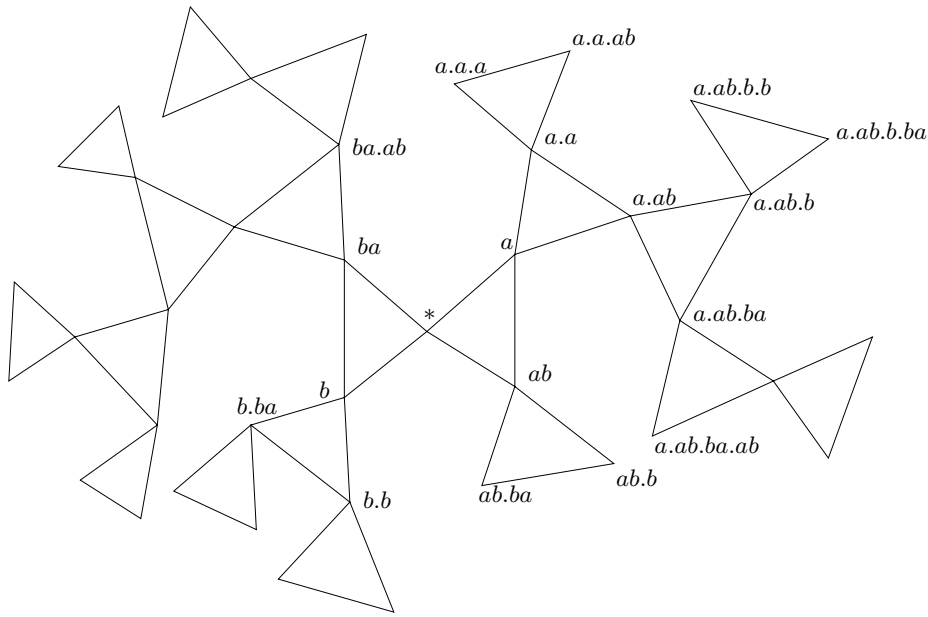
Figure 1: X(\mathcal{G}) for \mathcal{G} = \mathcal{A}/\Delta^2 , \mathcal{A} = \langle a, b \mid aba = bab \rangle
