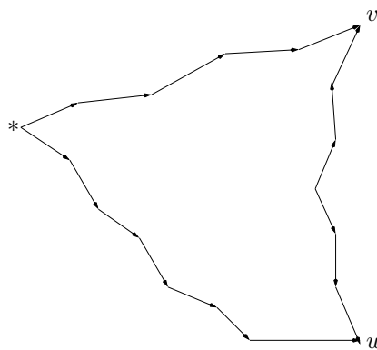
Figure 3: A geodesic triangle in X(\mathcal{G})
