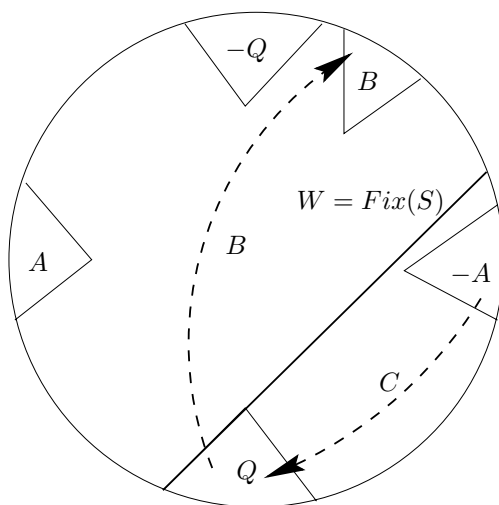
Figure 2: If W exists, C \cdot B is not a normal form; C can be extended to a geodesic gallery C' = Cs with C' < CB .
