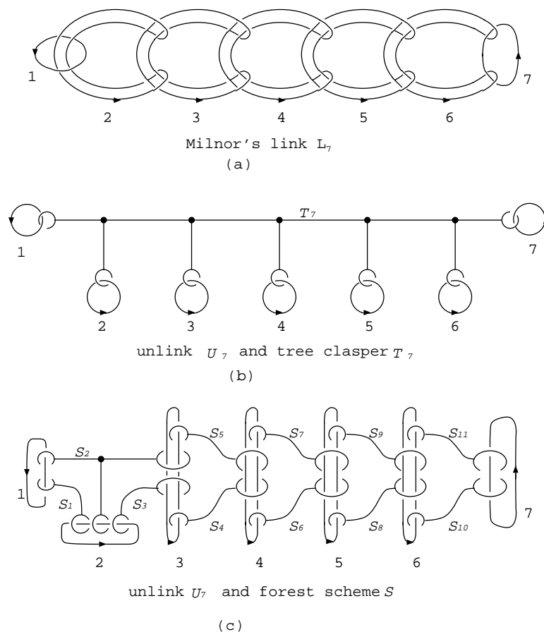
Figure 35: (a) Milnor's link L_7 of 7-components ( k = 6 ). (b) Strict tree clasper T_7 for the unlink U_7 . (c) Strict forest scheme S = S_1 [ \dots [ S_{11} for U_7 .
