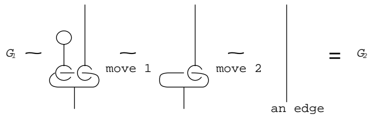
Figure 11: Proof of move 3
