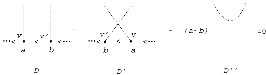
Figure 48: Let D be a uni-trivalent graph and let v < v^\theta be two consecutive univalent vertices in D labeled a, b \in H_1(\Sigma; \mathbf{Z}) . Let D^\theta be the uni-trivalent graph obtained from D by exchanging the order of v and v^\theta . Let D^{\theta\theta} denote the uni-trivalent graph obtained from D by connecting two vertices v and v^\theta . Then the "STU-like relation" states that D - D^\theta - (a \cdot b) D^{\theta\theta} = 0 , where a \cdot b \in \mathbf{Z} denote the intersection number of a and b . In this figure the univalent vertices are placed according to the total order.
