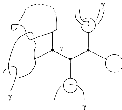
Figure 19: An example of a tree clasper T for a link in a 3-manifold M . Leaves of T may link with other leaves, and may run through any part of the manifold M .
