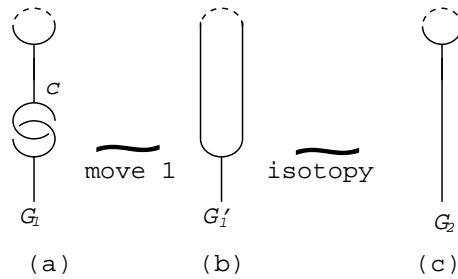
Figure 10: Proof of move 2
