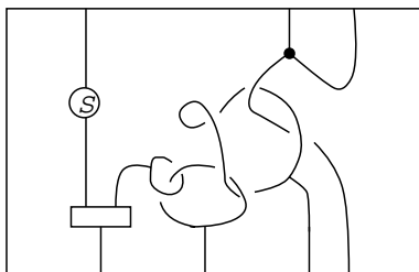
Figure 39: A clasper diagram representing a morphism from 3 to 4 in the category \mathbf{Cl}_0 .
