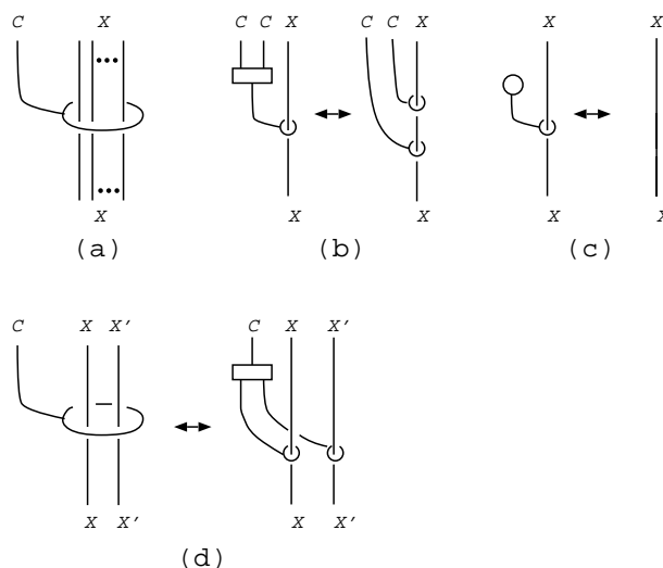
Figure 42: In (b), (c) and (d), the arcs labeled X and X^\theta represents parallel families of edges and strings (but not leaves). (a) Action of C on X . (b) Associativity. (c) Unitality. (d) Action on tensor product.
