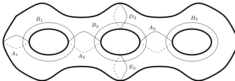
Figure 3: Supporting curves for a genus three positive relation
