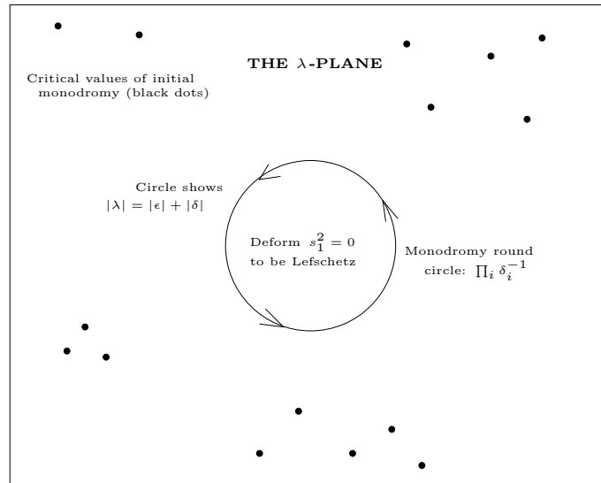
Figure 1: Stabilisation viewed in the \lambda -plane
