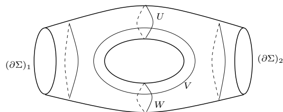
Figure 2: Supporting curves for a basic relation in \Gamma_{1,2}
