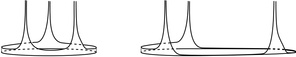
Figure 1: If c is a simple closed geodesic in S which is disjoint from a nonfilling geodesic lamination \mu , and if c is peripheral in S - \mu , then S - (\mu \cup c) has a component E whose metric completion \overline{E} is a crown. For each \epsilon > 0 , if c is sufficiently long then the set of points in c that are within distance \epsilon of \partial\overline{E} - c consists of at least 1 - \epsilon of the total length of c .
