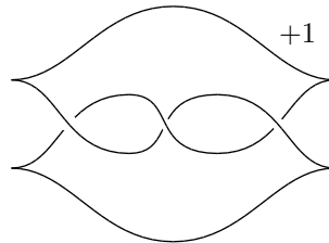
Figure 1: A contact structure on -\Sigma(2, 3, 4)
