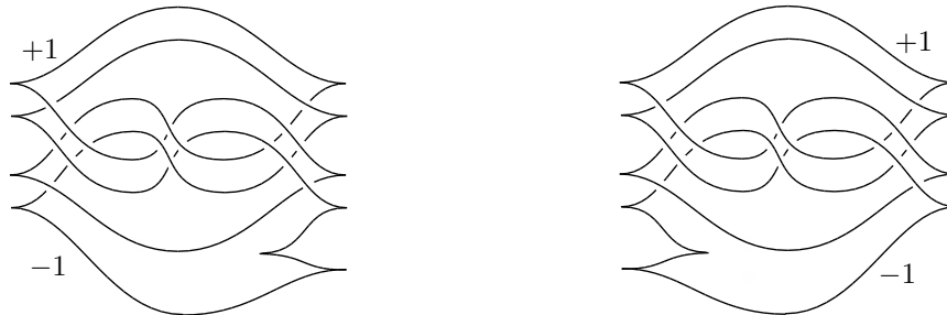
Figure 2: Contact structures on -\Sigma(2, 3, 3)
