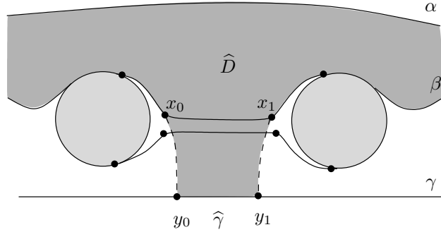
Figure 30: The shaded subdiagram \widehat{D} consists of the union of D_\alpha with the quadrilateral diagram \square with corners x_0, x_1, y_1, and y_0 .
