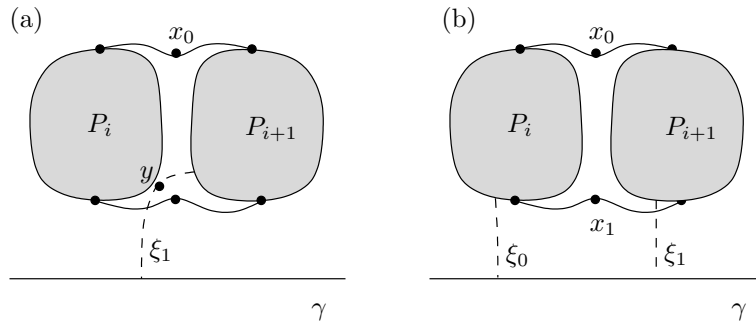
Figure 31: (a) The path \xi_1 intersects C_0 . (b) For each j \in \mathbb{Z}_2 , the path \xi_j intersects C_j .
