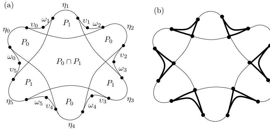
Figure 24: (a) The convex hull of the union of two intersecting preflats (b) The darkened triangles are \delta -thin.
