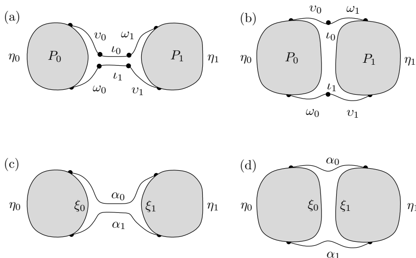
Figure 22: The convex hull of two disjoint preflats P_0 and P_1 . In (a), the Hausdorff distance between \iota_0 and \iota_1 is at most \delta . In (b), each \iota_i has image a single point. In (c) and (d) the quadrilateral bounded by \xi_0 , \alpha_0 , \xi_1 , and \alpha_1 is \delta -thin. The two pictures indicate the two possible shapes of a thin quadrilateral.
