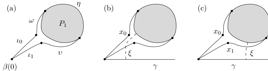
Figure 27: (a) The convex hull of the preflat P_1 and the point \beta(0) (b) The path \xi intersects \iota_1 . (c) The path \xi intersects \eta\nu .
