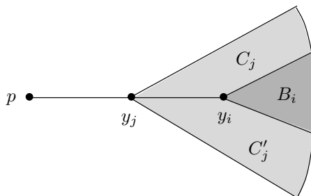
Figure 19: Two shadows that intersect
