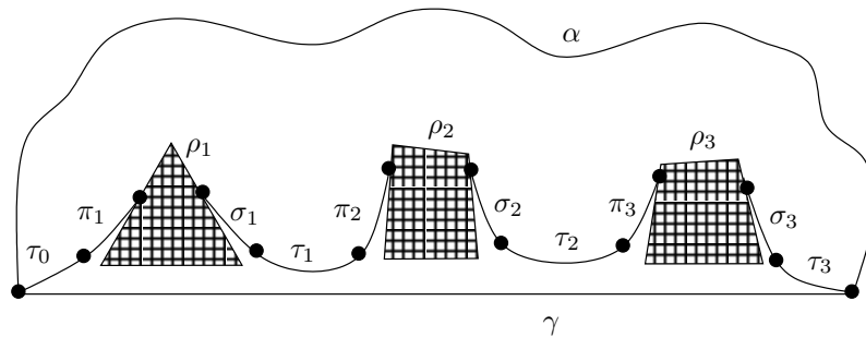
Figure 26: The path \beta stays close to the union of the preflats in \mathcal{P} and \text{Im}(\gamma) .
