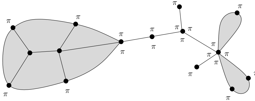
Figure 7: Formally place an angle of size \pi at each corner of S^2 - D . The curvature at a vertex is 2\pi minus the angle sum of all corners at v including these “exterior” corners.
