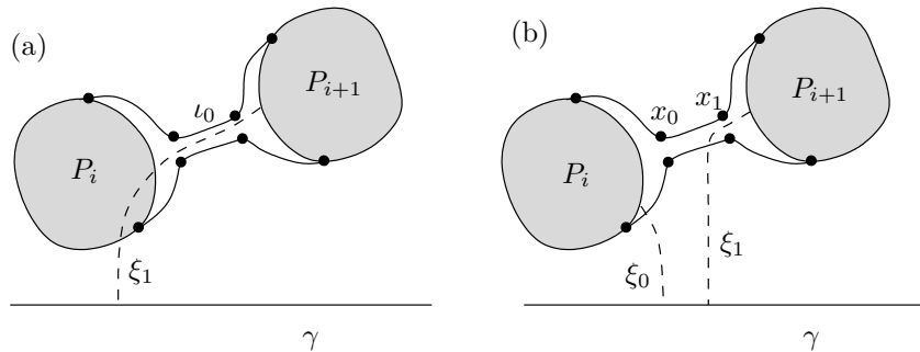
Figure 29: (a) The path \xi_1 intersects C_0 . (b) For each j \in \mathbb{Z}_2 , the path \xi_j intersects either C_j or \iota_1 .
