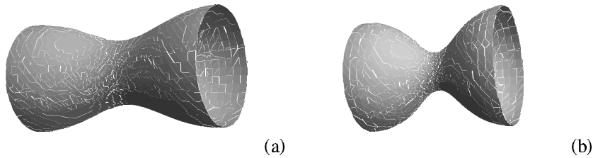
Figure 2. Unduloid-like surfaces obtained using the parametric equations (24) and (26) for: (a) p/k_c = 0.6962 , (b) p/k_c = 1.1250 .
