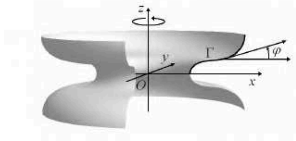
Figure 1. Sketch of a surface of revolution obtained by revolving around the z -axis a plane curve \Gamma laying in the xOz -plane, which is defined by the graph (x, z(x)) of a function z = z(x) . Here, \varphi is the (tangent) slope angle.
