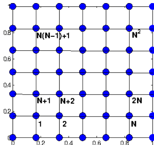
Figure 3.1: Lexikographic numbering of vertices of the equidistant tensor product mesh.
